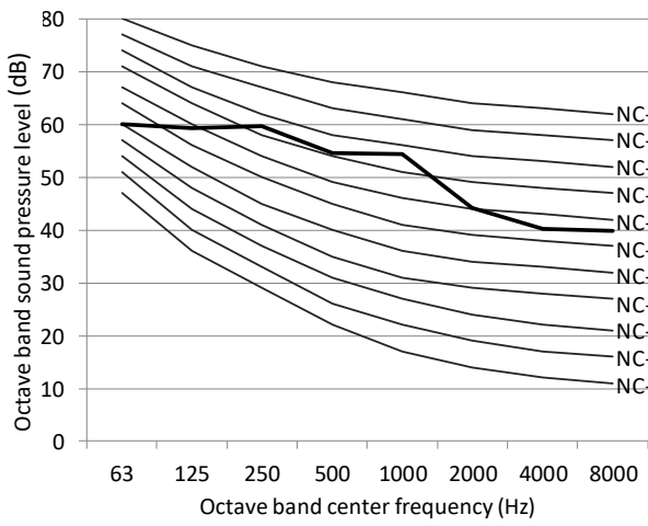
Figure 2-10.3 8/10HP octave band level
