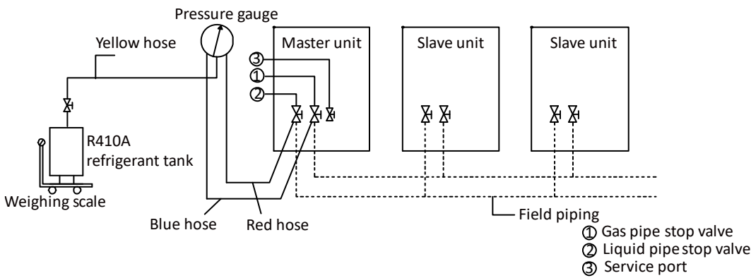
Figure 3-8.1: Charging refrigerant
