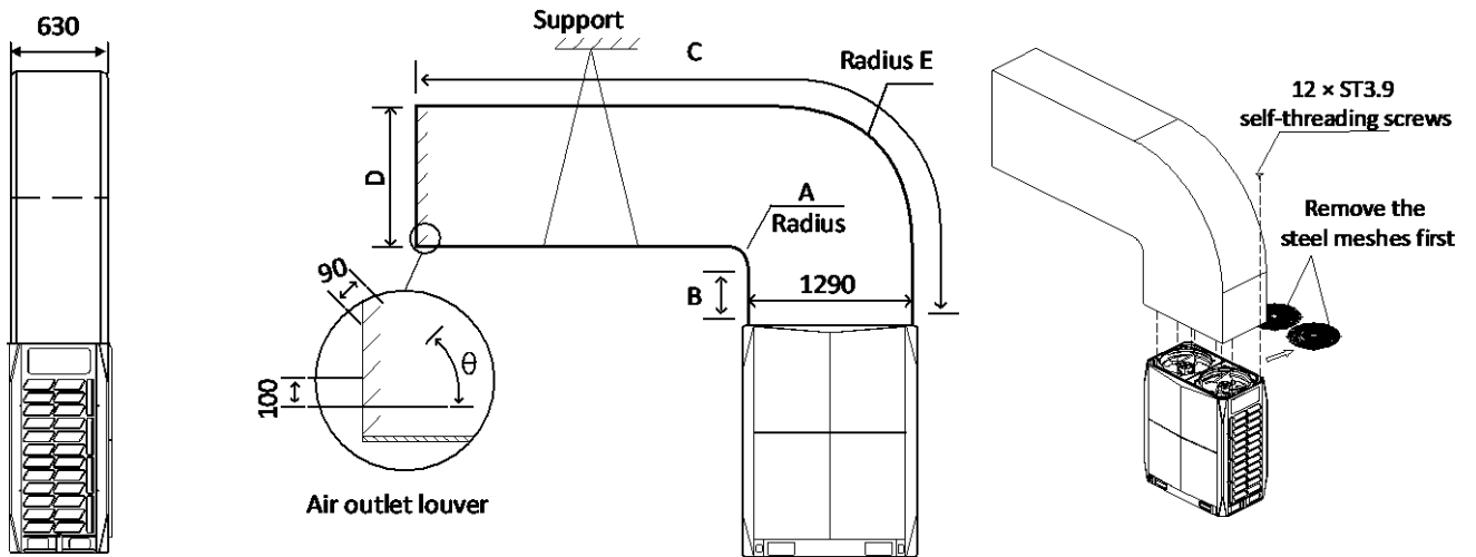
Figure 3-3.7: Longitudinal ducting for 18HP, 20HP and 22HP units (unit: mm)
