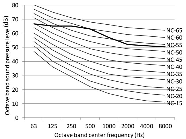
Figure 2-10.8 24HP octave band level
