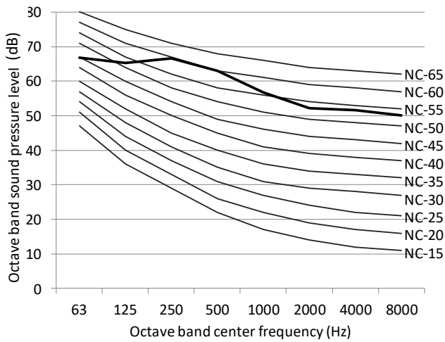
Figure 2-10.9 26/28/30/32HP octave band level
