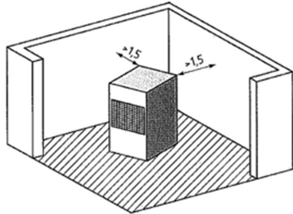
Figure 2-10.2: Sound power level measurement (unit: m)
