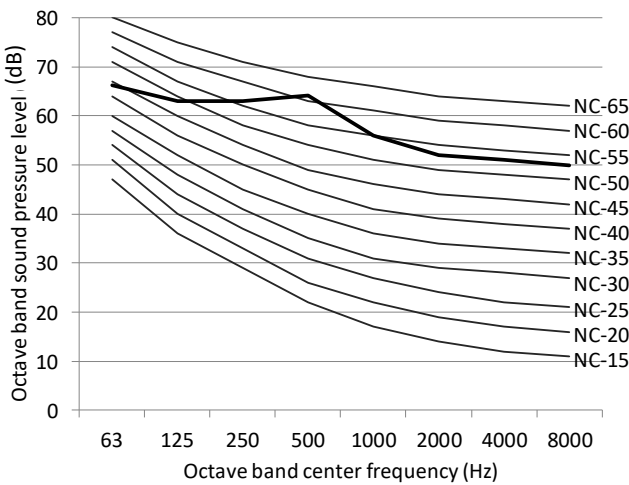
Figure 2-10.7 20/22HP octave band level
