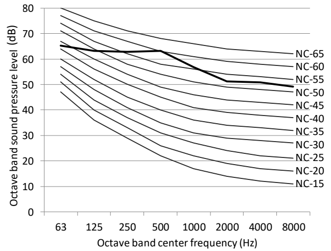
Figure 2-10.6 16-18HP octave band level
